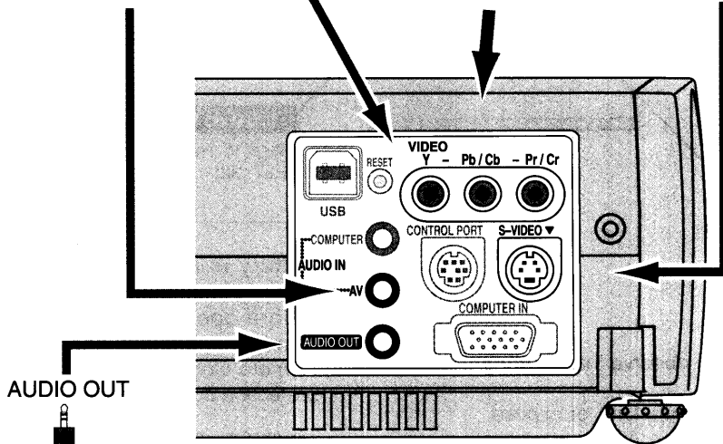
Terminals of the Projector
