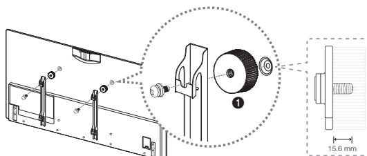
Case B. Installing another company's Wall-Mount
